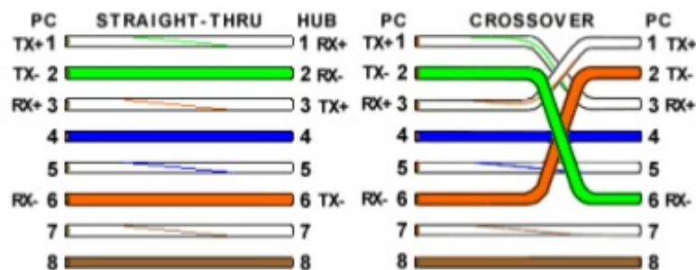
Figure 1: Straight and Cross cable connections
